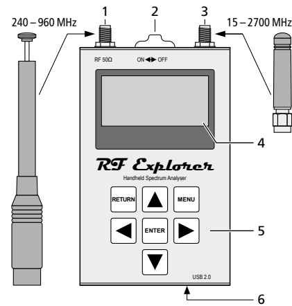
Fig. 1 Connections and operating elements
