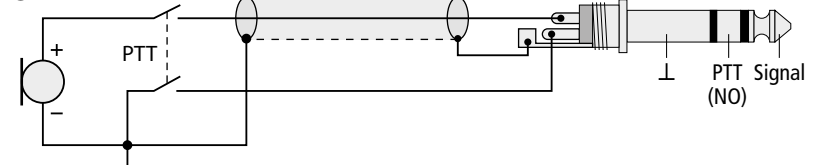
② DH-95NP
