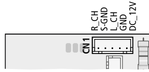
PCB with connectors
